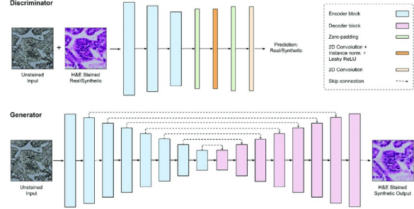
Fig. 3: Model Architecture
