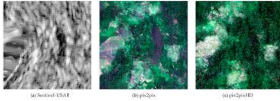
Fig. 2: Data Pre-Processing
