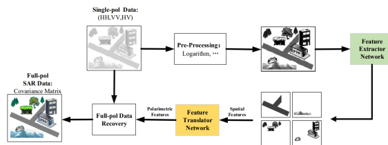
Fig. 1: framework for automatic SAR image colourisation
